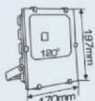
PHA LED 005 - 30W ●○ 933.000
