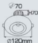
AFC PULY 02 LED 10W 536.000
